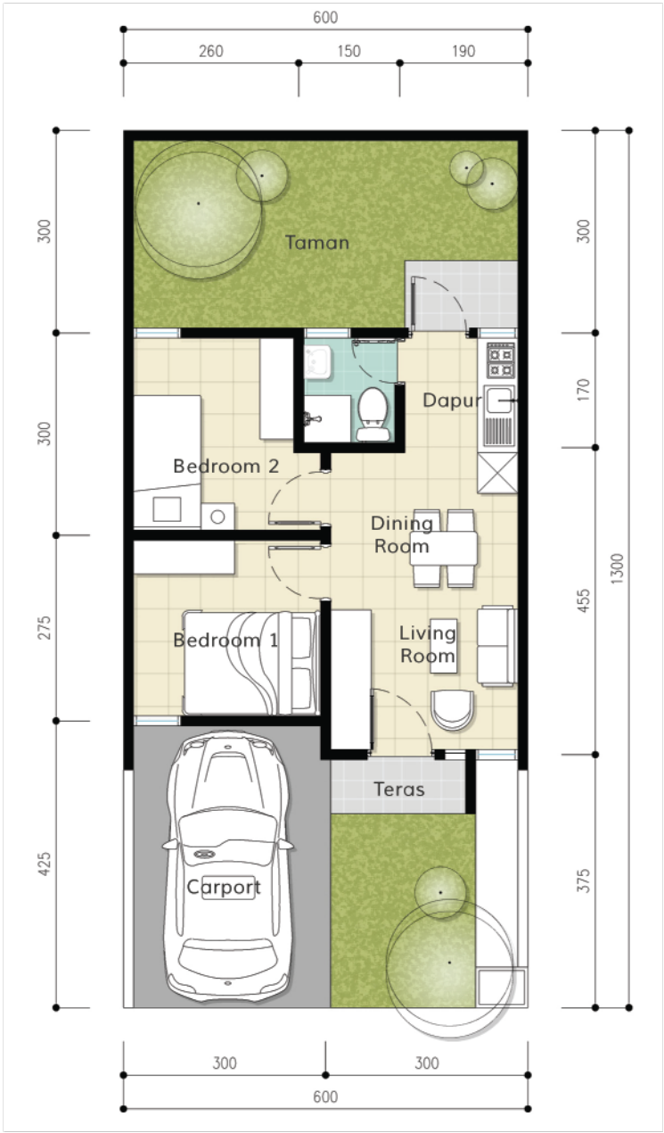
Denah Lantai 1 LB. 41 M2 / LT. 78 M2
